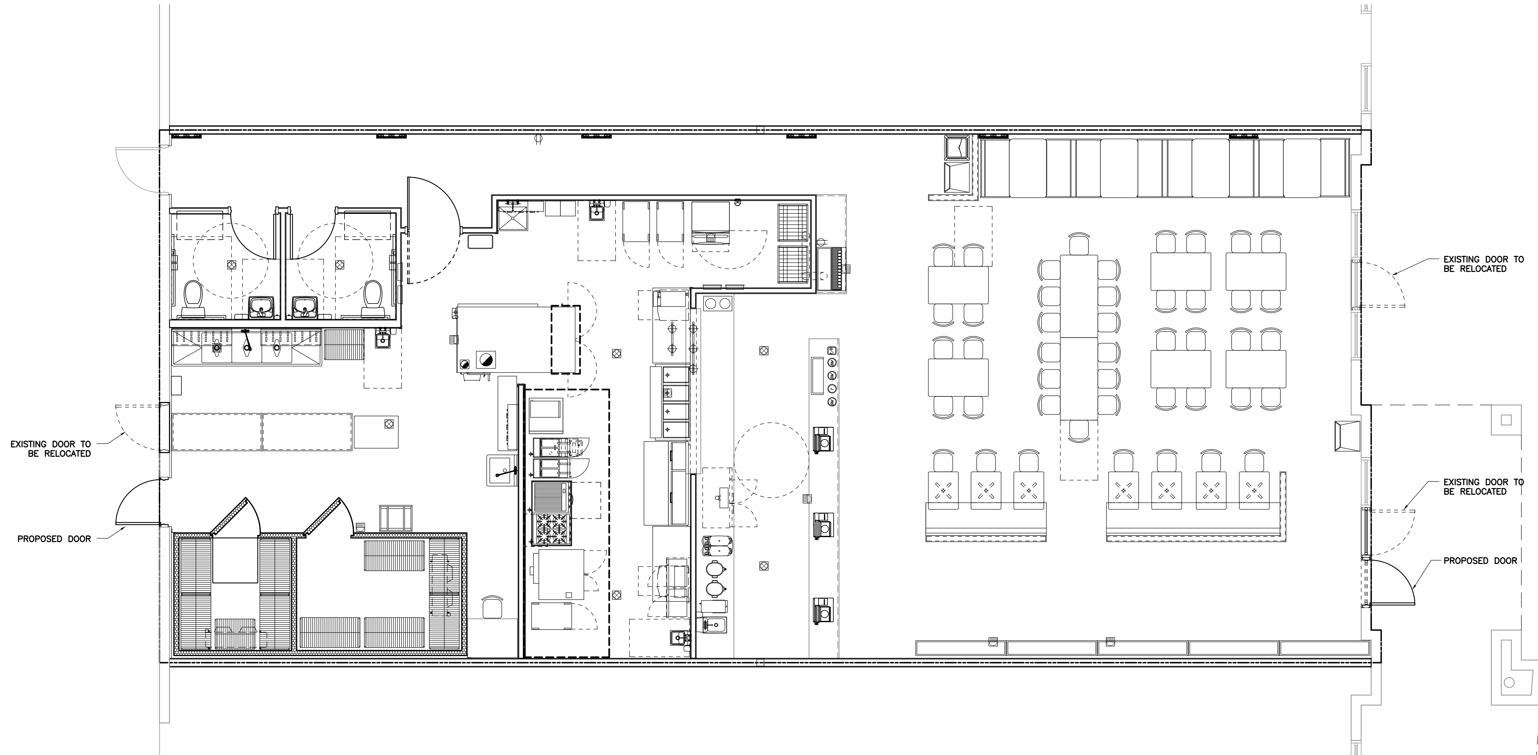
01 PROPOSED FLOOR PLAN - scheme B February 6, 2013 SCALE: 1/4" = 1'-0"
